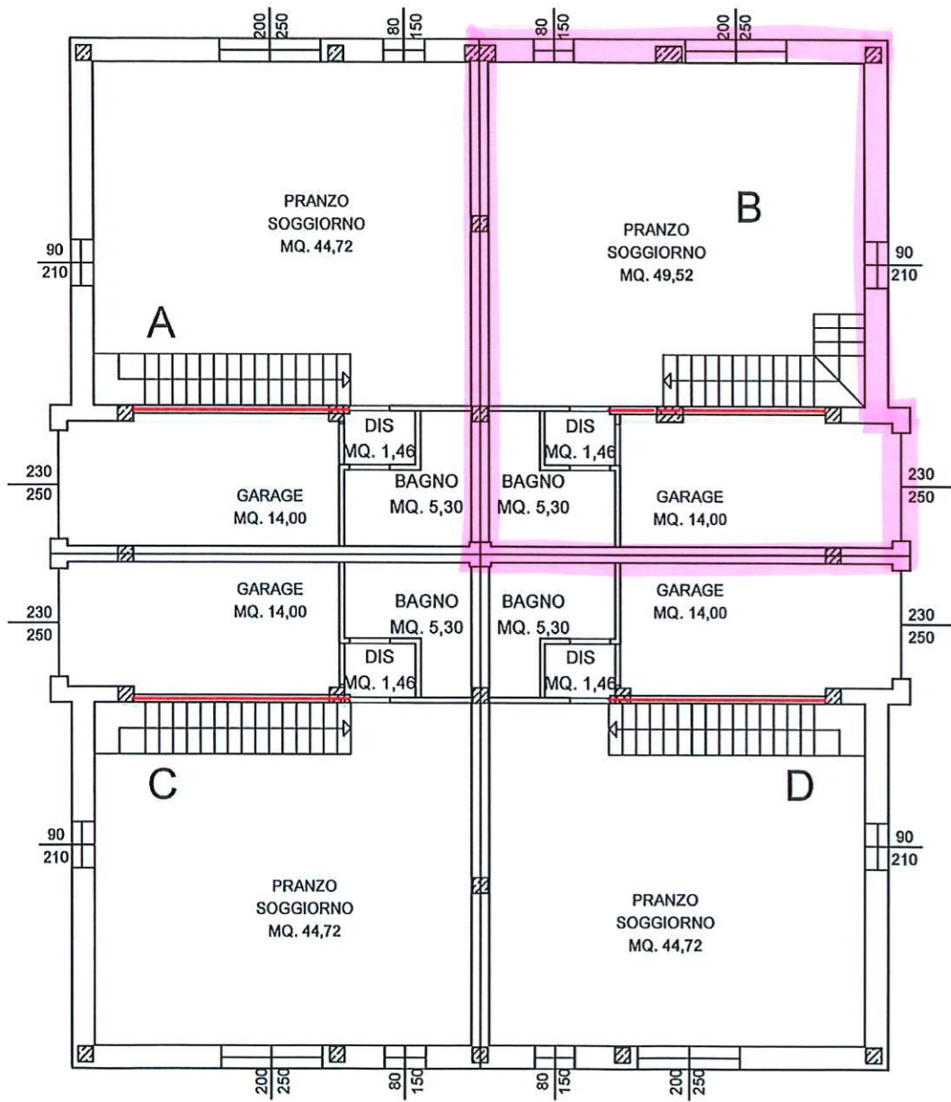
PIANO TERRA
